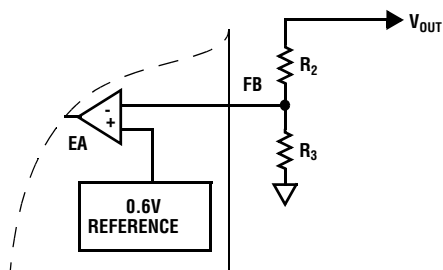
FIGURE 45. EXTERNAL RESISTOR DIVIDER
